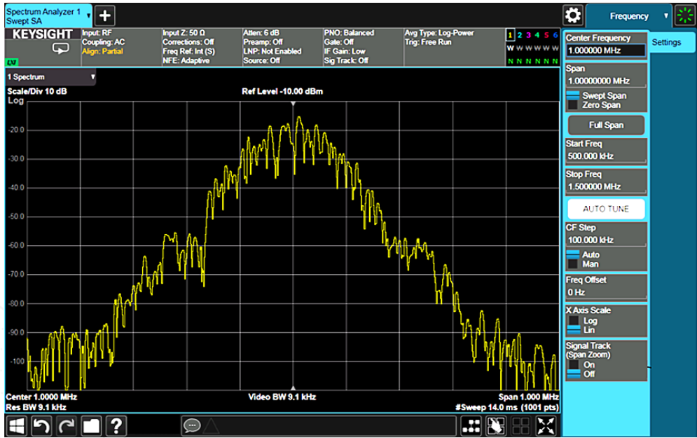
Figure 2-41. Spectrum of the GSM signal
