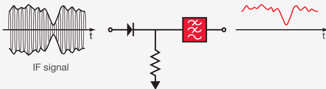
Figure 2-16a. Envelope detector
