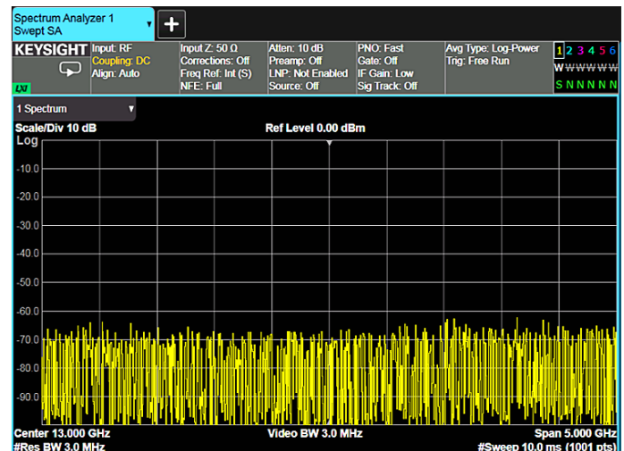
Figure 2-23b. Sample mode
