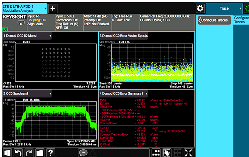
Figure 8-6. EVM measurement of LTE FDD downlink signal
