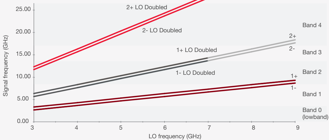
Figure 7-7. X-Series analyzer harmonic bands using LO doubling
