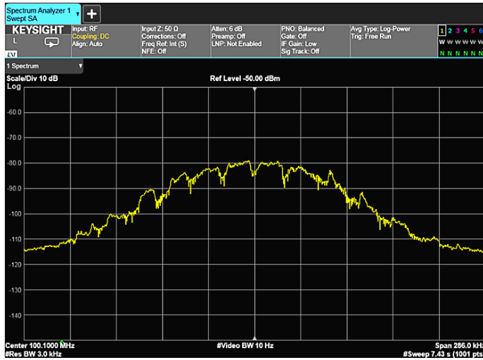
Figure 2-32a. Video filtering
