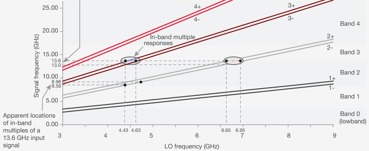
Figure 7-5. Tuning curves up to 4th harmonic of LO showing in-band multiple responses to a 13.6-GHz input signal
