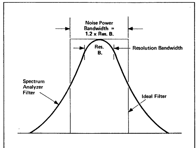
Figure 2. Comparison of Real & Ideal Filter Response showing the Equivalent Noise Power Bandwidth.
