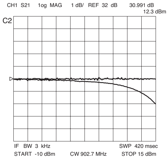
Figure 4. 1-dB Compression
