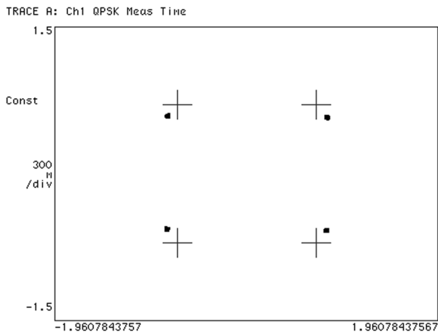
Figure 20. I/Q Gain Imbalance (excess I gain and reduced Q gain relative to the ideal constellation locations)
