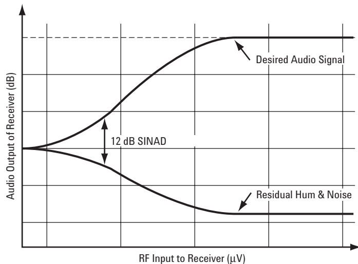
Figure 8. Understanding SINAD
