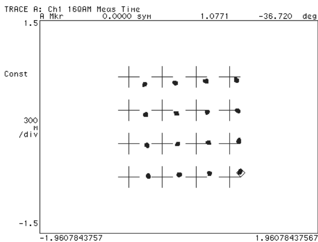
Figure 22. I/Q Offset
