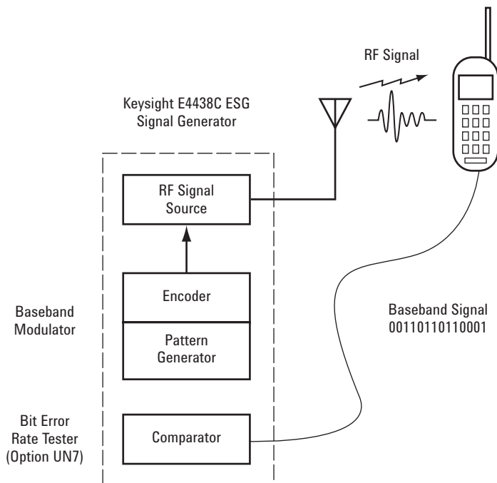
Figure 6. Baseband BER Test Configuration
