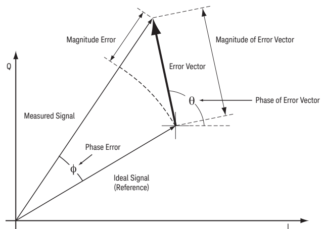
Figure 29. EVM and Related Quantities
