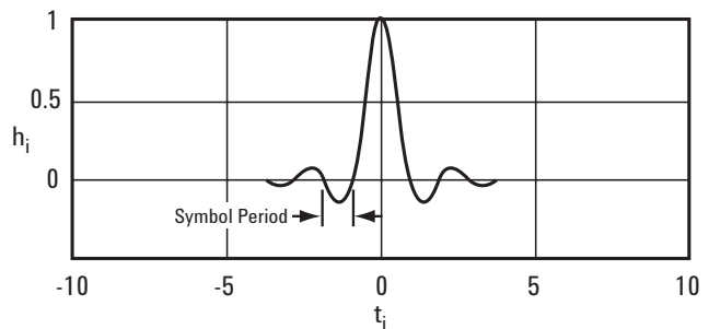
Figure 5. Impulse Response of a Nyquist Filter
