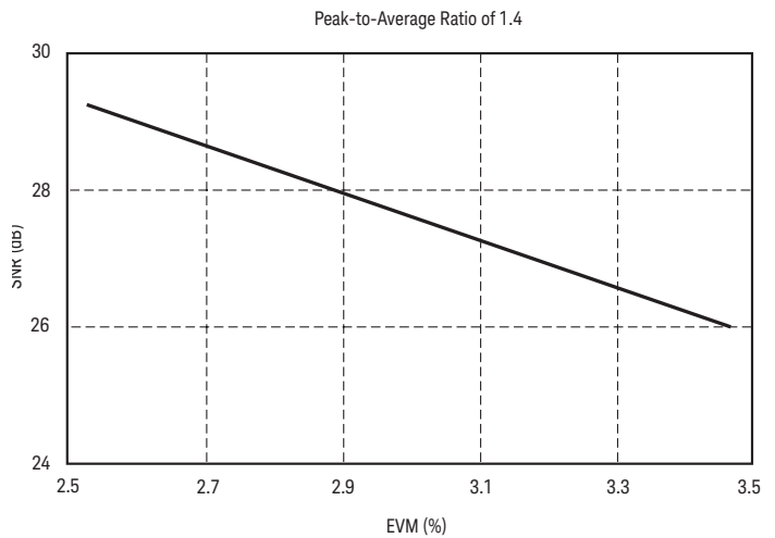
Figure 31. SNR Versus EVM for Crest Factor of 1.4
