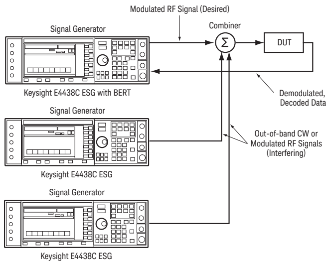
Figure 13. Intermodulation Immunity Measurement Setup
