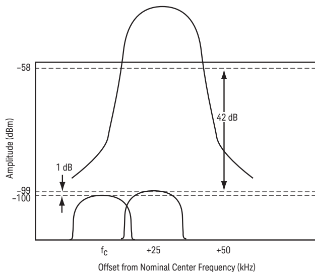
Figure 18. PDC Adjacent and Alternate Channel Selectivity Spectrum
