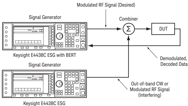
Figure 11. Spurious Immunity Measurement Setup
