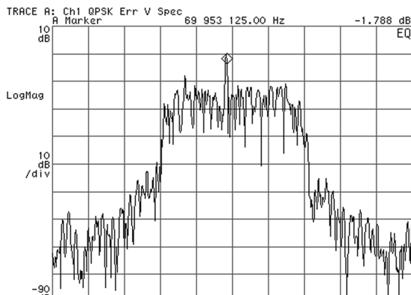
Figure 24. Error Vector Spectrum Reveals Spur
