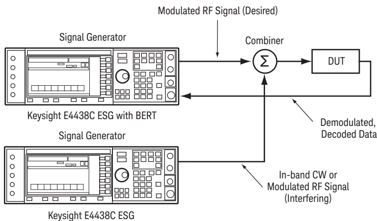
Figure 10. Co-Channel Rejection Measurement Setup
