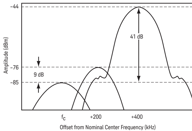
Figure 16. GSM Adjacent and Alternate Channel Selectivity Spectrum
