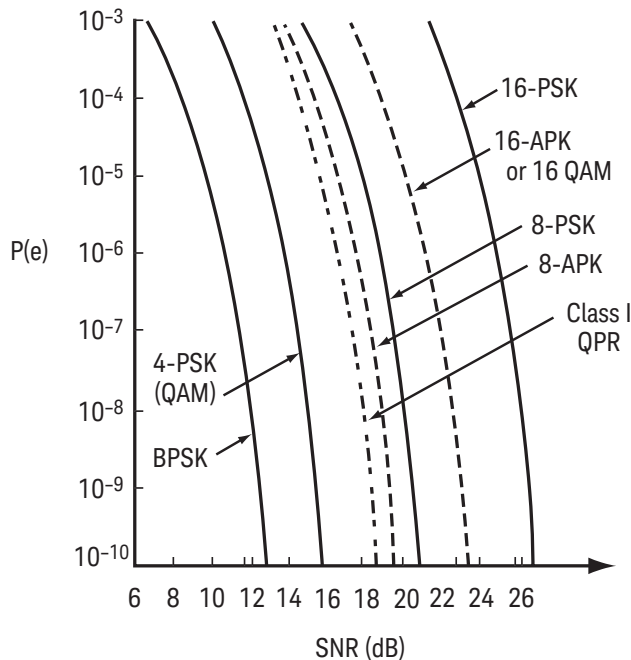
Figure 30. Probability of Error Versus SNR
