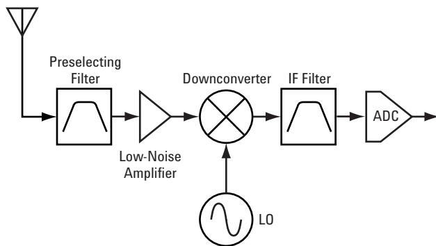
Figure 4. Sampled IF Receiver
