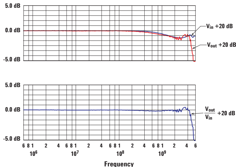
Figure 8. (Top) Frequency response of V_{in} and V_{out} of the Keysight 1158A, 4 GHz probe. (Bottom) Since the frequency response of V_{out} closely tracks V_{in} , the transmitted response of the probe remains flat throughout the 4 GHz bandwidth of the probe.
