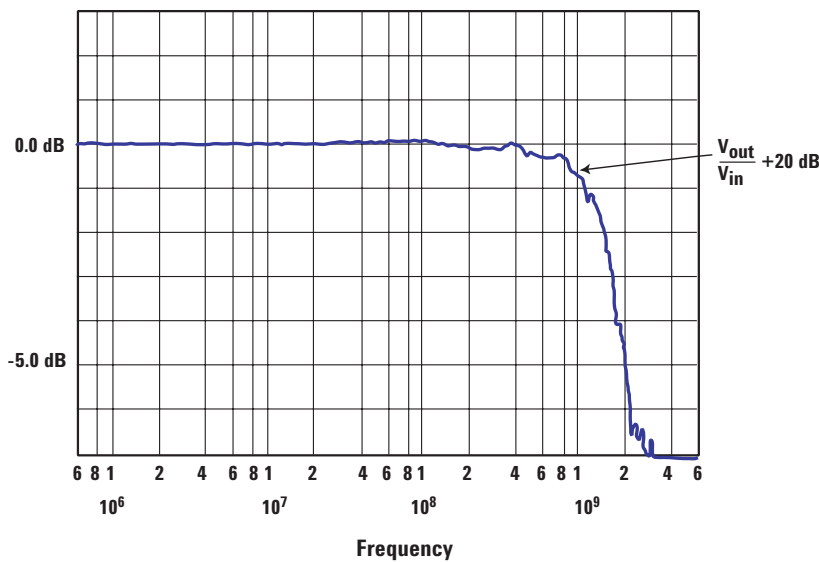
Figure 11. Probing with the 5-cm resistive signal leads for the Keysight 1158A probe will reduce the bandwidth of the measurement, but the transmitted response remains flat and no distortion is introduced into the measured waveform.
