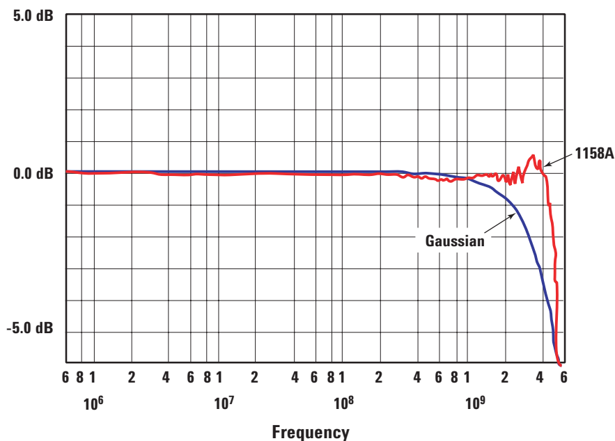
Figure 13. Comparison of Gaussian transmitted response and the steep roll-off of the Keysight 1158A probe.
