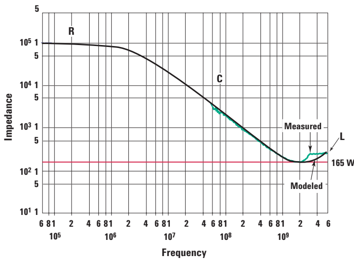
Figure 4. Increasing frequency changes the input impedance of the Keysight 1158A probe.
