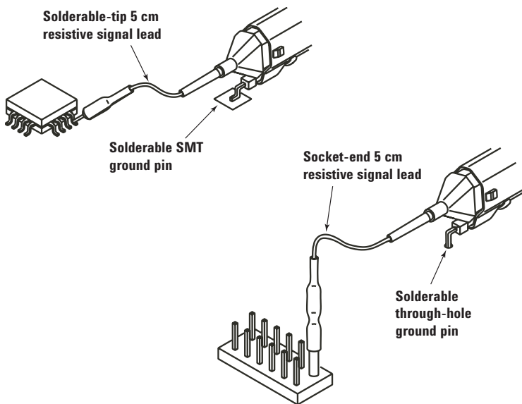
Figure 10. Probing with the Keysight 1156A/57A/58A probes and properly damped accessories increases measurement reliability.
