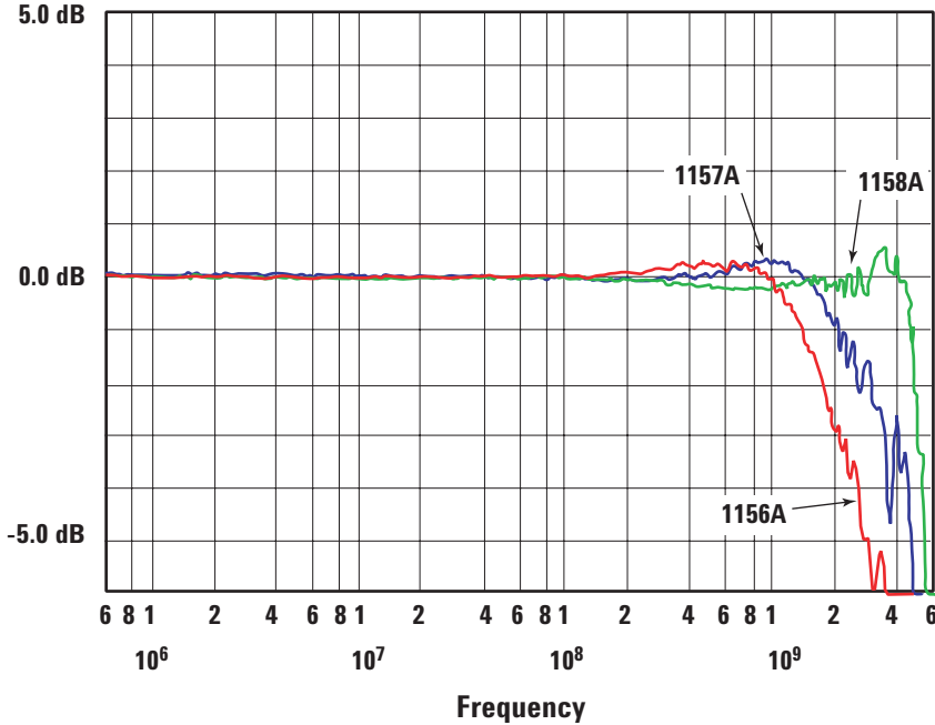
Figure 14. Transmitted response of the Keysight 1156A (1.5-GHz), 1157A (2.5-GHz), and 1158A (4-GHz) probes.
