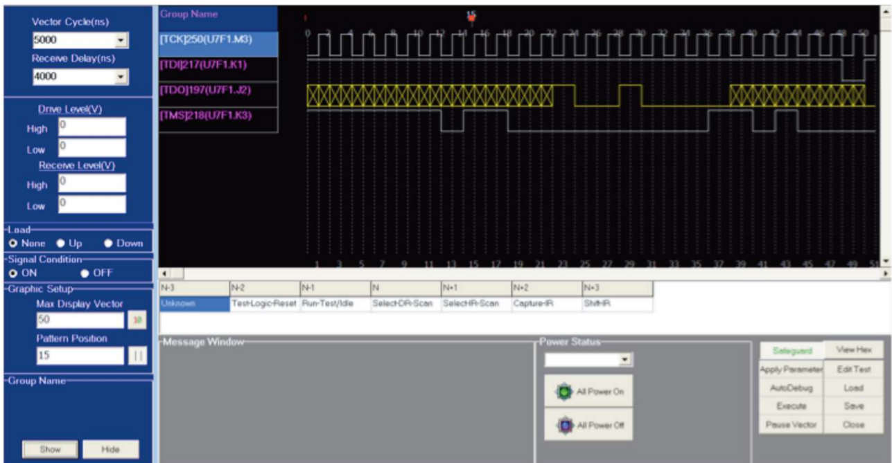
Figure 2. Digital Debugging is made easy on the Medalist i1000D with graphical interface.
