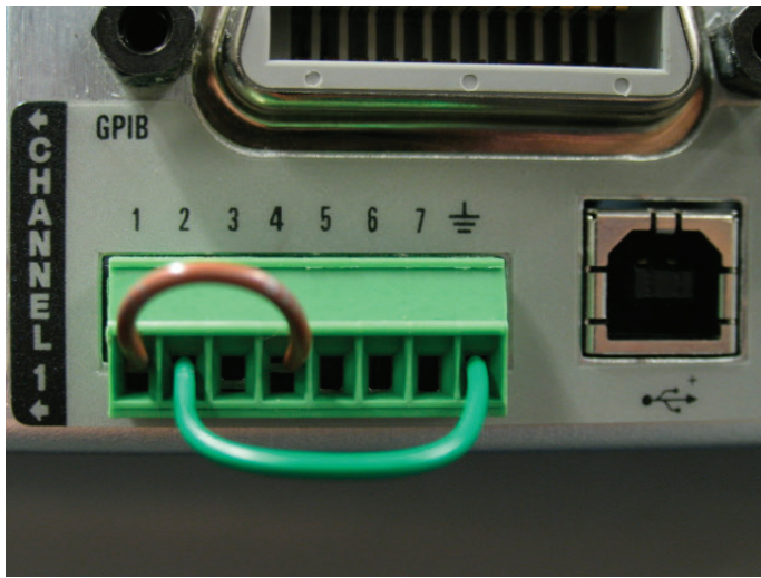
Figure 3a. 8-pin digital port connector wiring for single mainframe
