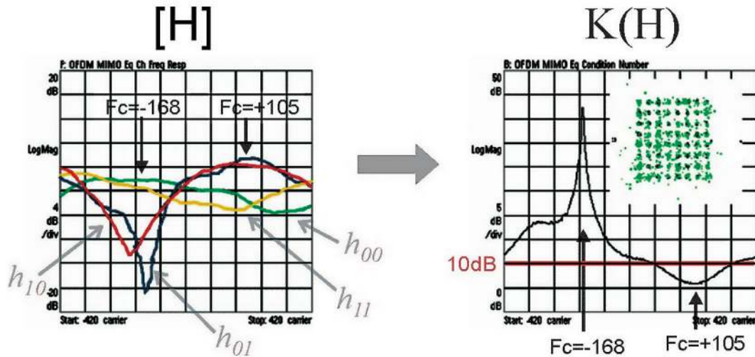
Figure 3. Measurements of the four channel coefficients and associated condition number as a function of subcarrier frequency for an LTE 2x2 MIMO signal. Note the measured channel responses are normalized while the condition number is calculated from the complex channel coefficients before normalizing.
