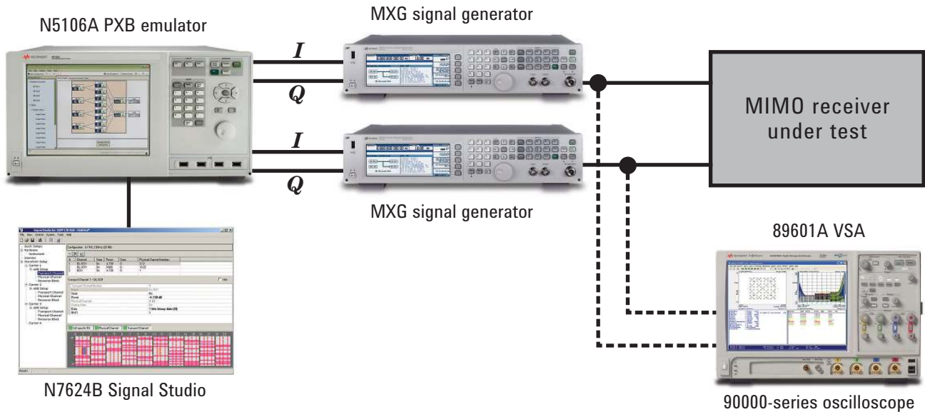
Figure 8. Measurement configuration for testing the performance of a 2x2 MIMO receiver under a variety of multipath conditions.
