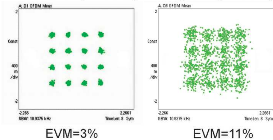
Figure 4. Measured constellation and EVM performance for an LTE 2x2 MIMO system having low and high condition numbers.
