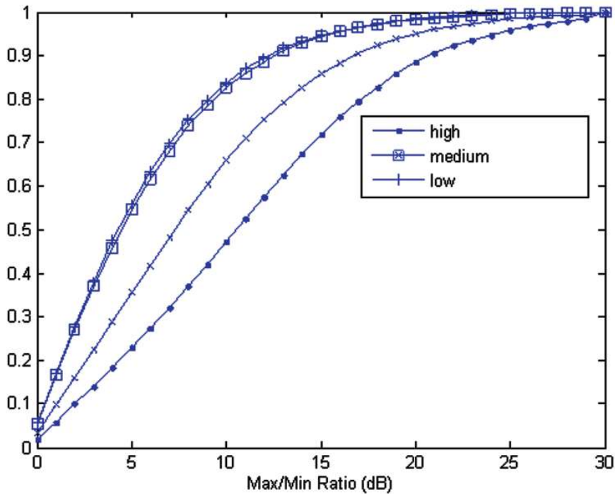
Figure 7. Cumulative Density Function (CDF) for the condition number as a function of correlation between the channel coefficients.
