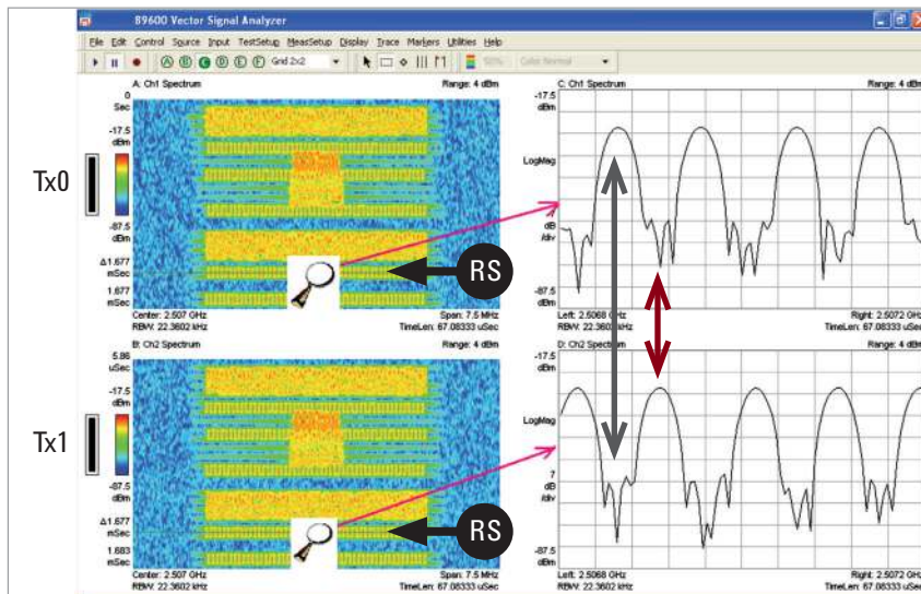
Figure 2. Measurements of the spectrograms and frequency responses for a LTE 2x2 MIMO signal. The upper spectrogram measurement, shown on the left, is for the signal transmitted from antenna Tx0 and the lower plot from antenna Tx1. The time-gated spectrums, shown on the right, display the orthogonal RS (pilot) subcarriers used for estimating the channel coefficients. The measurements were made using the Keysight 89601A VSA using a Hanning window with a time constant set to match the symbol length.
