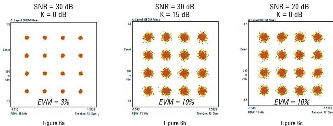
Figure 6. Measured constellation and associated EVM for a 2x2 MIMO system operating under various SNR and channel conditions. For Figure 6a, the SNR equals 30 dB and channel is ideal. For Figure 6b, the SNR is 30 dB and condition number is 15 dB. For Figure 6c, the SNR is 20 dB and channel is ideal.
