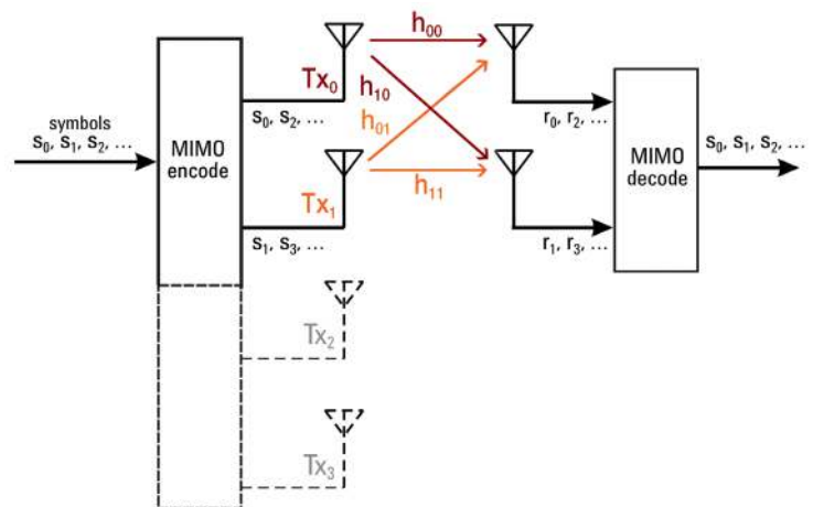
Figure 1. Basic 2x2 MIMO system using spatial multiplexing and having four channel matrix coefficients. Also shown is the option for two additional transmitter antennas creating a 4x2 configuration. Note for the 4x2 case, the channels coefficients are not shown.
