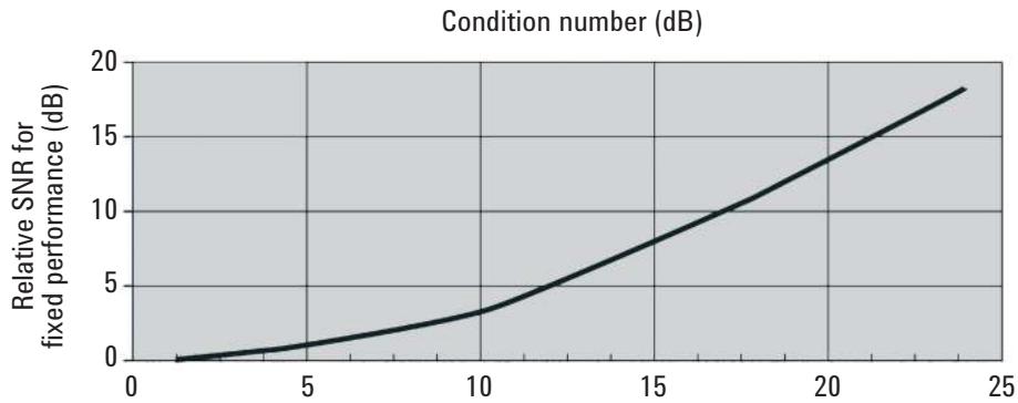
Figure 5. Empirical relationship between the MIMO condition number and the relative SNR required to achieve the same level of performance in MIMO and SISO systems.
