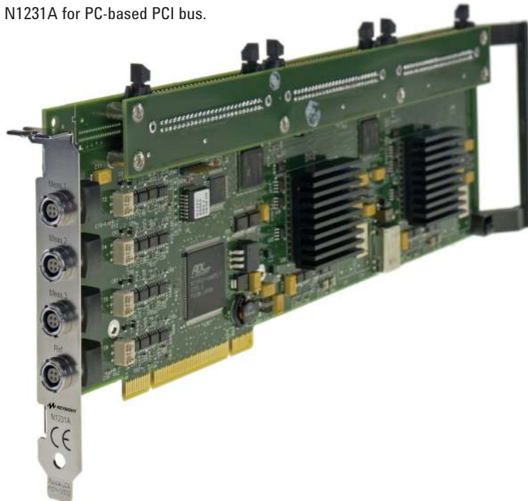
Figure 3. Keysight electronics solutions are available for multiple platforms and include the N1225A VMEbus and the N1231A for PC-based PCI bus.
