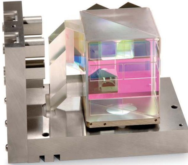
Figure 4. Keysight's multi-axis interferometers are designed and produced using our unique Complex Monolithic Optics (CMOs) technology and provide extreme precision and reliability in a compact form factor.
