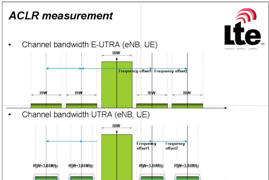
Figure 5. Two specified methods of ACLR measurement
