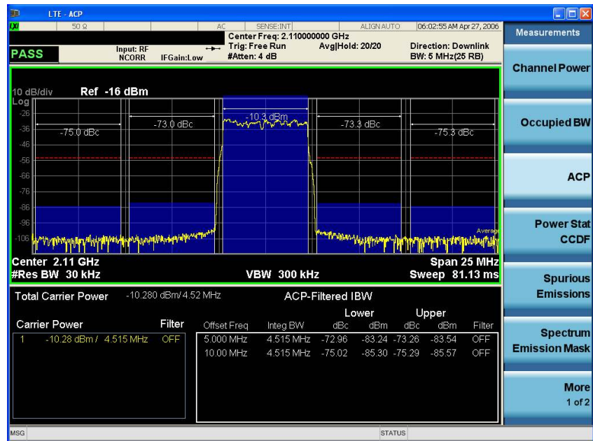
Figure 7. ACLR measurement result using Keysight X-series analyzer after optimization
