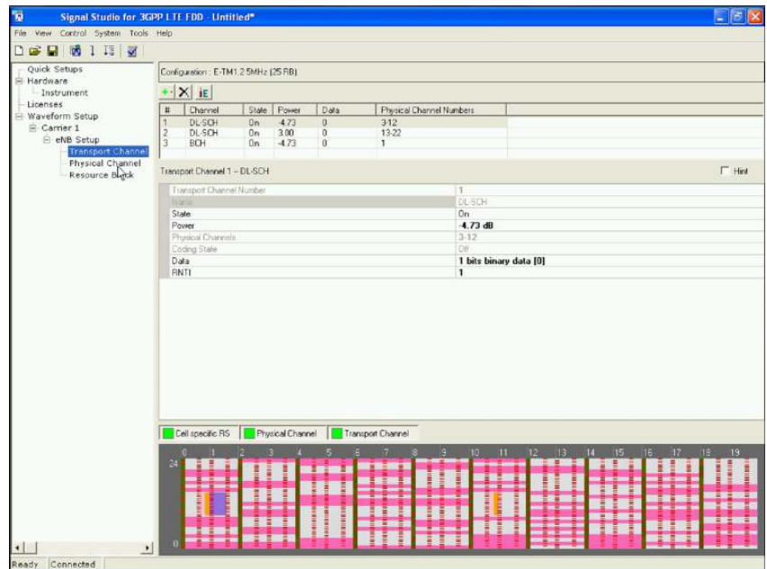
Figure 3. Resource allocation blocks (at bottom) for E-TM1.2 test signal
