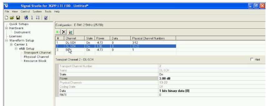
Figure 4. Boosted output power in Channel 2
