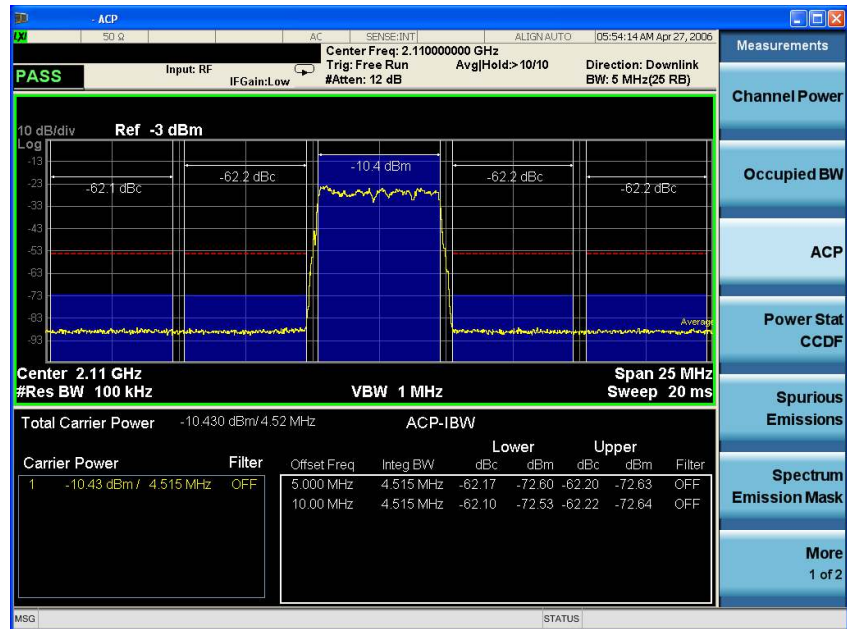
Figure 6. ACLR measurement result using Keysight X-Series analyzer before optimization
