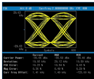
ASK/FSK modulation analysis (Option DMA)
