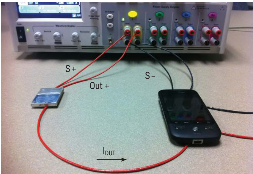
Figure 2: The actual setup for measuring battery run-down performance using the N6781A SMU installed as output 1 in an N6705B DC power analyzer mainframe.
