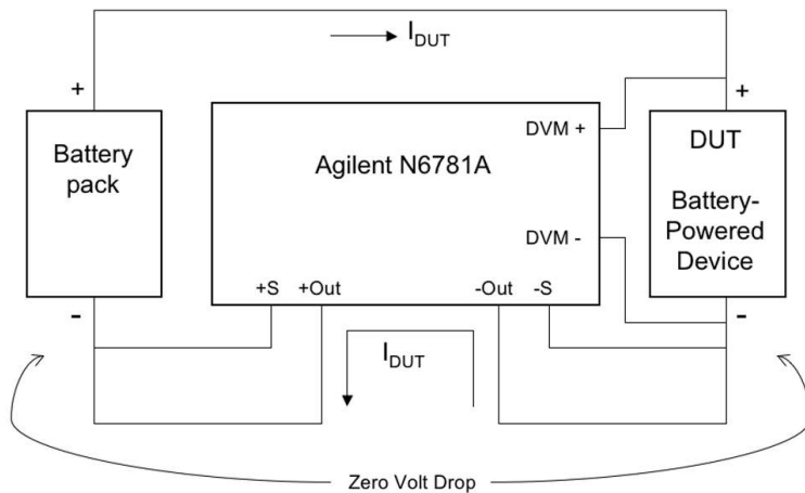
Figure 1: The recommended setup for measuring battery run-down performance using the N6781A SMU. Note that remote voltage sensing eliminates the voltage drop in the wiring between the battery pack (-) and DUT (-). In this setup, the N6781A SMU module will be installed inside an N6705B DC power analyzer mainframe.
