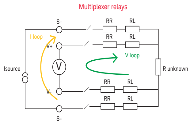
Figure 4. 4-wire technique where one loop provides current to R_{\text{unknown}} , creating a voltage drop, measured in the low current V loop. The current in the V loop is small due to the high impedance of the voltmeter, therefore RR and RL can be neglected and R_{\text{unknown}} is accurately measured.
