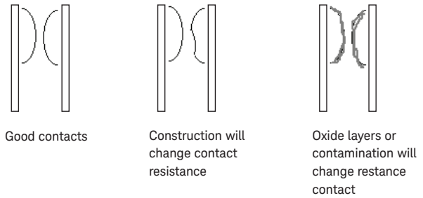
Figure 8. Relay contacts.
