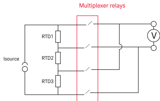
Figure 7. Series RTD configuration with external current source.
