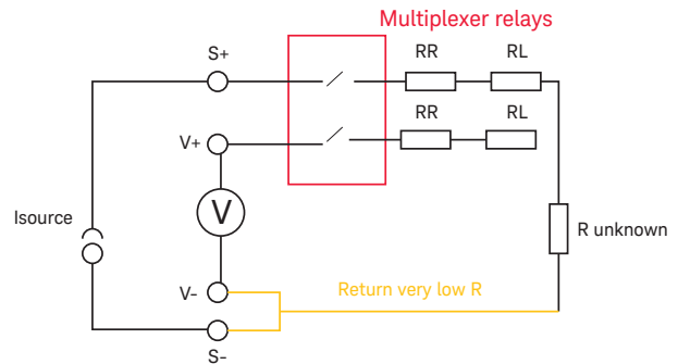
Figure 5. Three-wire technique.
