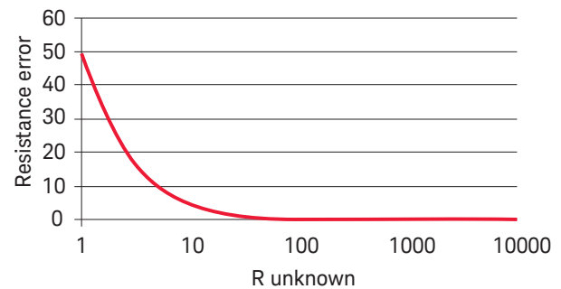
Figure 3. Two-wire error.
