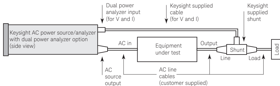
Figure 1. Test configuration of efficiency measurement using an Keysight AC source with the O20 dual power analyzer option.
