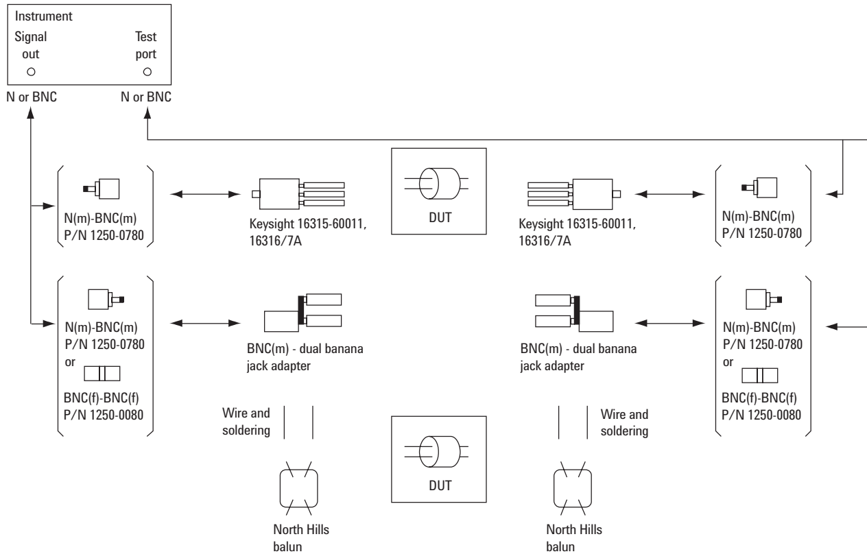
Figure 7. Measurement configuration (3)
