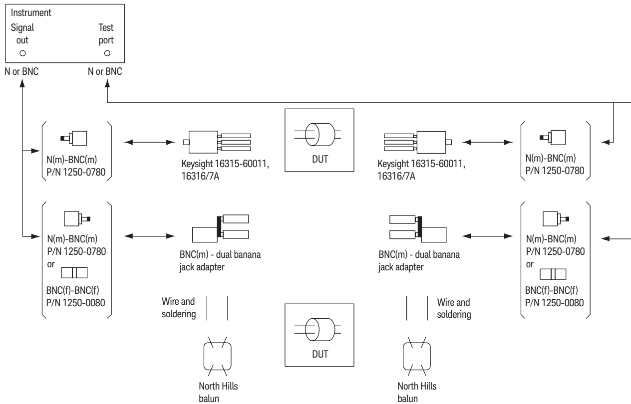
Figure 7. Measurement configuration (3)
