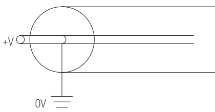
Figure 2. Unbalanced cable
