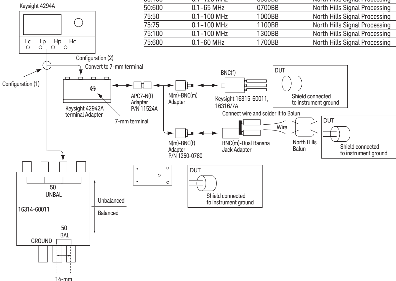
Figure 4. Measurement configurations with 4294A
