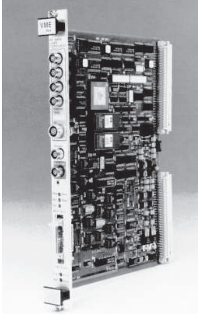
Improve system accuracy and repeatability using Keysight 10896B VMEbus laser compensation electronics.
