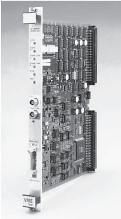
Get the highest positioning accuracy and repeatability available with the Keysight 10897B High Resolution Laser Axis Board for VMEbus.
