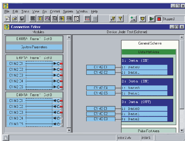
Figure 5: The Connection Window helps you to create a virtual model of your measurement set-up
