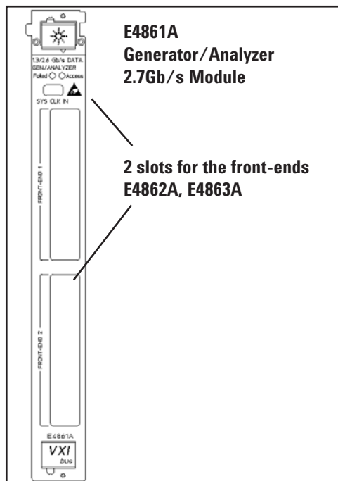
Figure 14: E4861A Module
