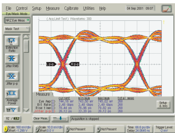
Figure 13a) b): Signal of E4861A with E4862A and E4863A Analyzer
