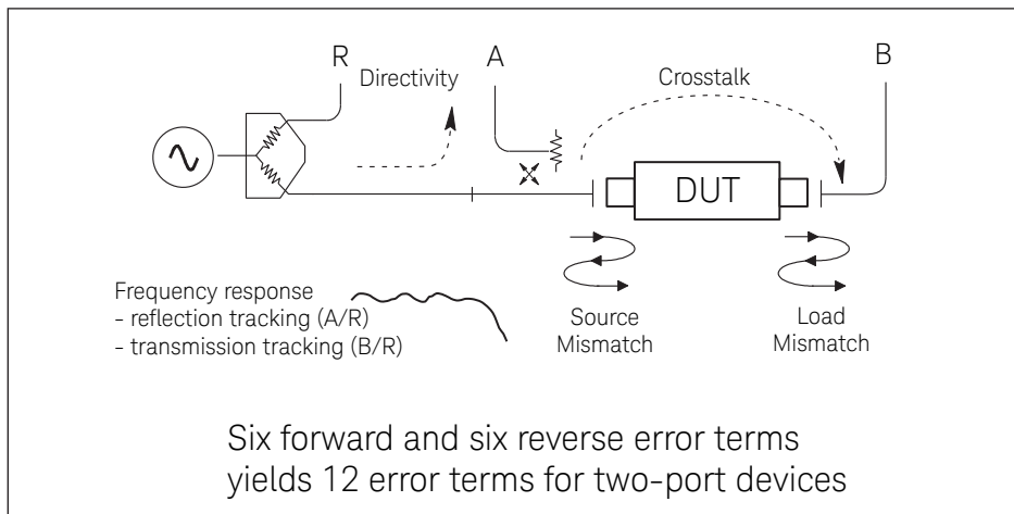
Figure 2. Systematic Measurement Errors
