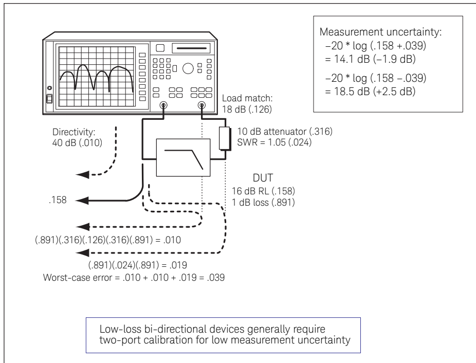
Figure 9. Relection Example using a One-port Cal plus an Attenuator
