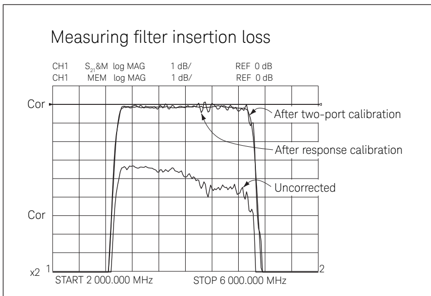
Figure 1. Response versus Two-Port Calibration
