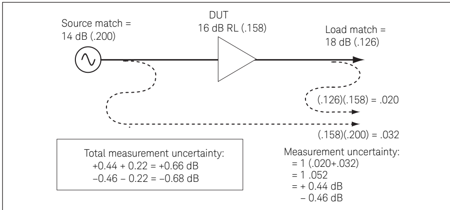
Figure 12. Measuring Amplifiers with a Response Calibration
