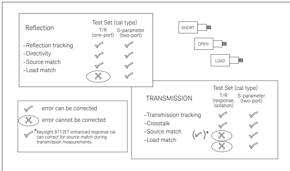
Figure 7. Calibration Summary
