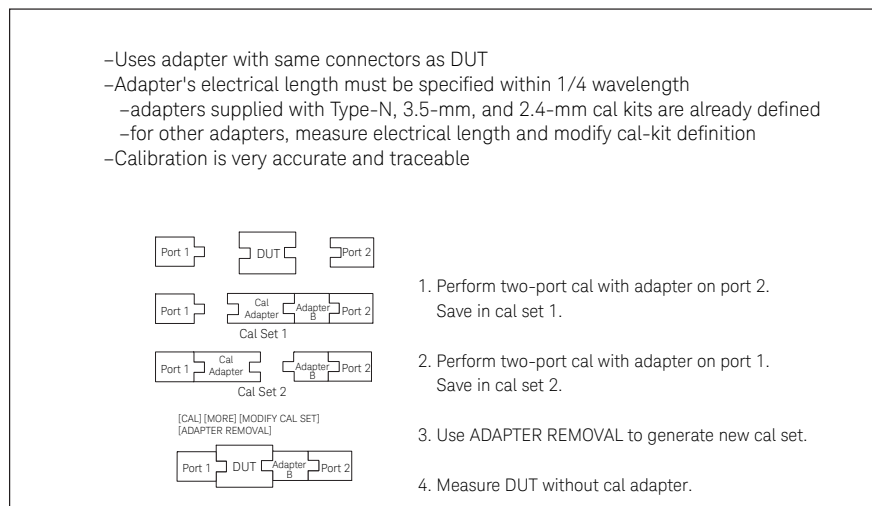
Figure 15. Adapter-Removal Calibration
