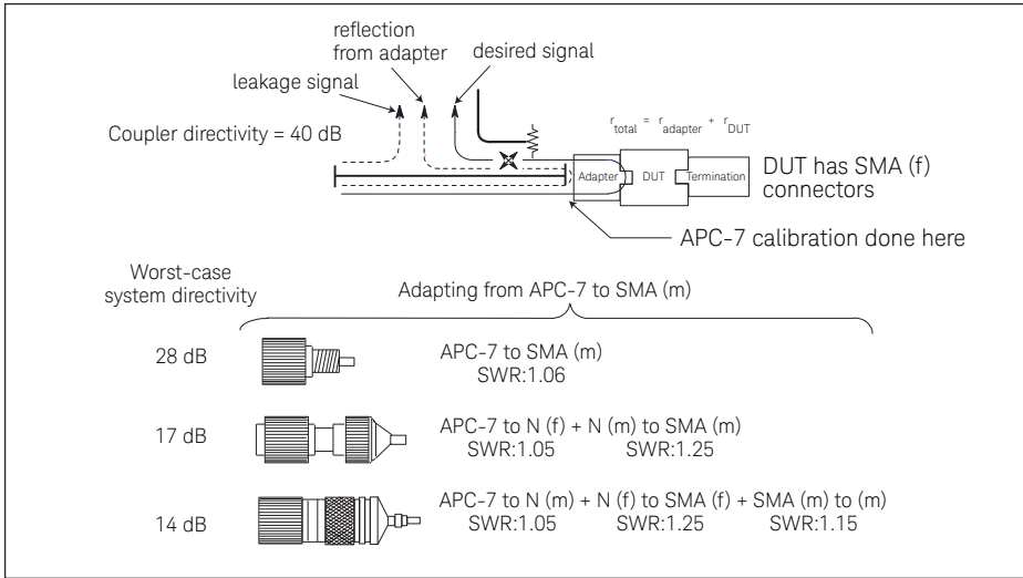
Figure 4. Adapter Considerations
