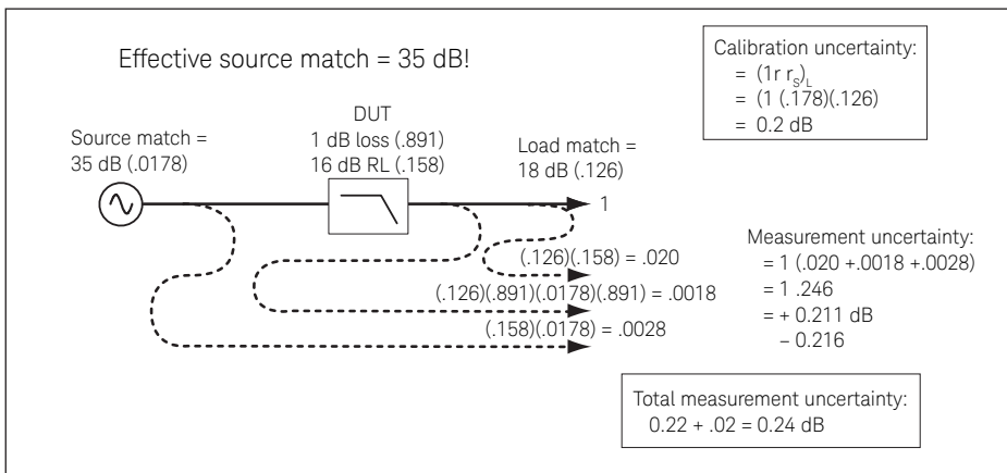
Figure 13. Transmission Measurements using the Enhanced-Response Calibration
