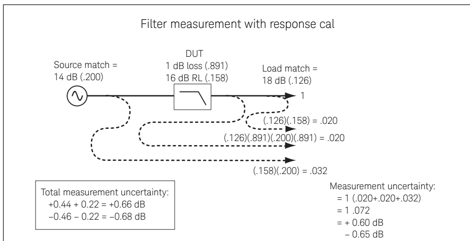
Figure 11. Transmission Example (continued)
