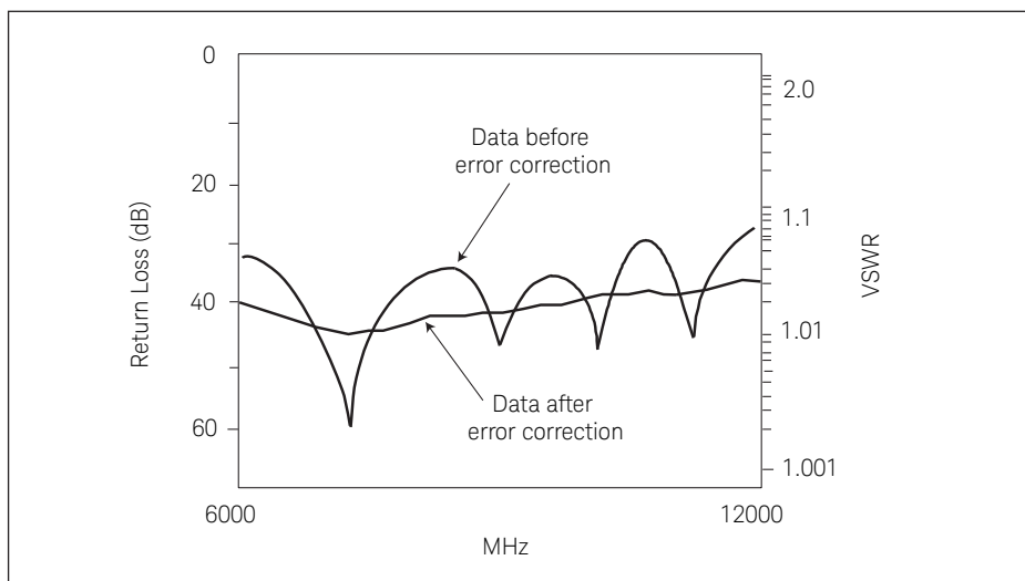
Figure 3. Before and After One-Port Calibration
