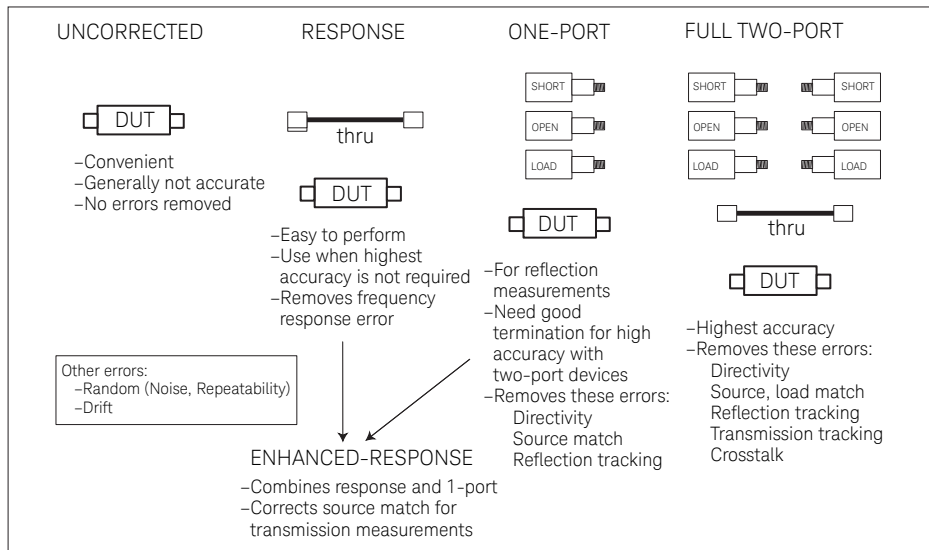
Figure 6. Errors and Calibration Standards
