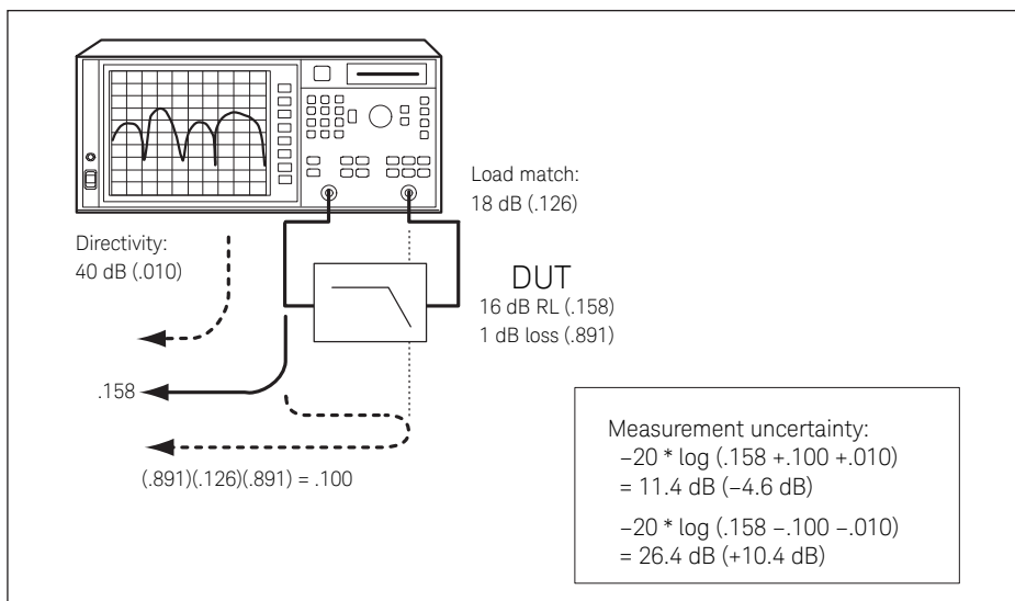
Figure 8. Reflection Example Using a One-Port Cal
