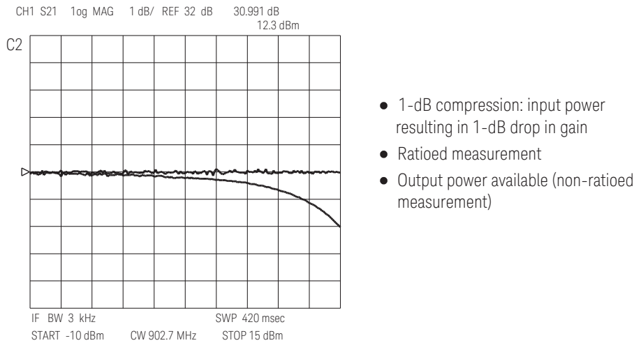
Figure 4. 1-dB Compression
