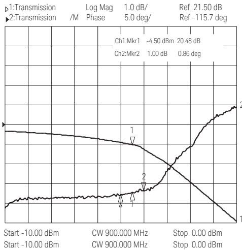
Figure 5. AM-to-PM Conversion
