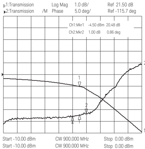
Figure 5. AM-to-PM Conversion
