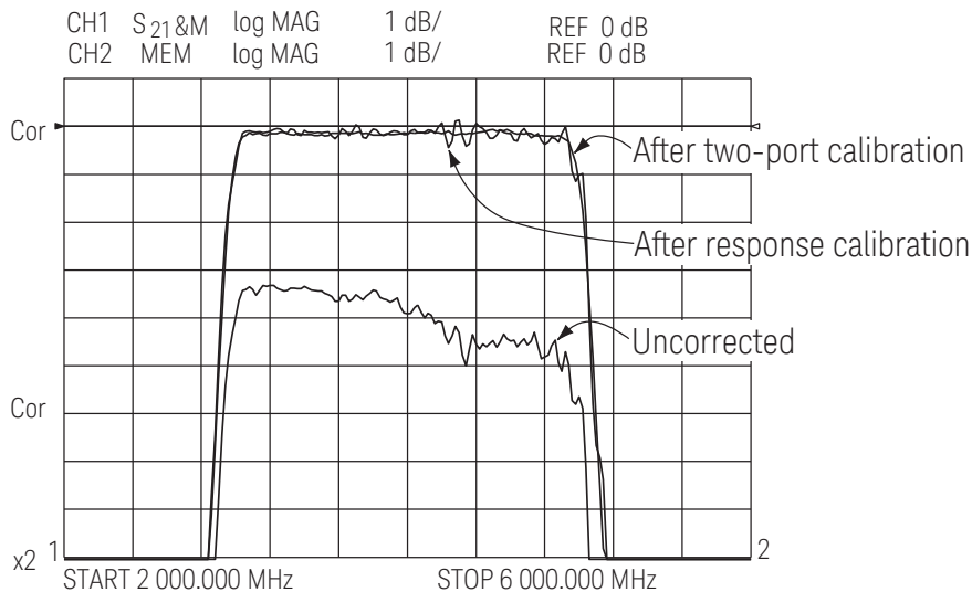
Figure 2. Systematic Measurement Errors
