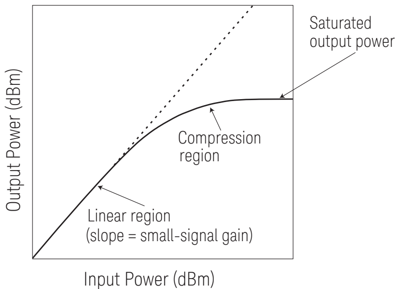
Figure 3. Power Sweeps Characterize the Compression Region
