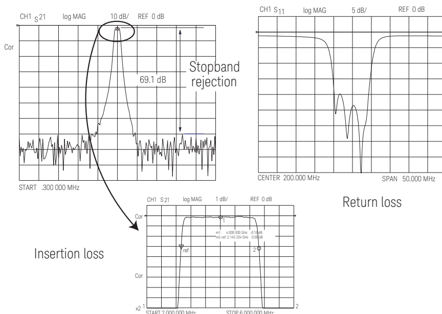
Figure 1. Testing Filters with Frequency Sweeps
