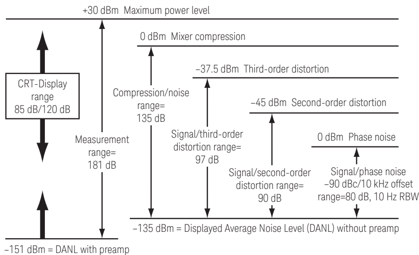
Figure 1. Dynamic range interpretations
