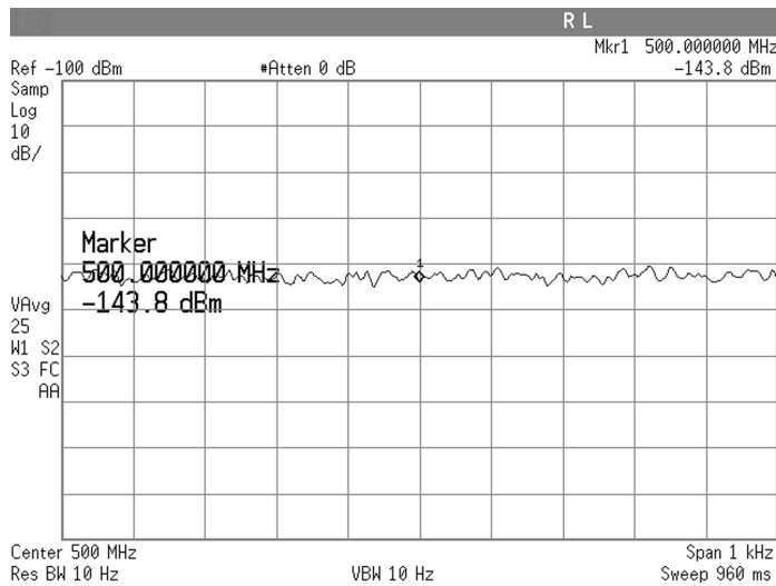
Figure 6. DANL of an Keysight ESA-E series spectrum analyzer without preamplification
