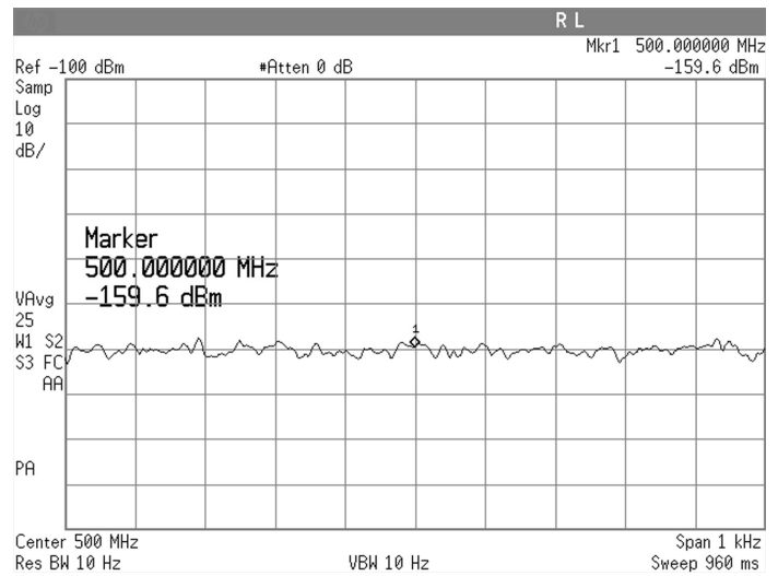
Figure 7. DANL of an Keysight ESA-E series spectrum analyzer with preamplification
