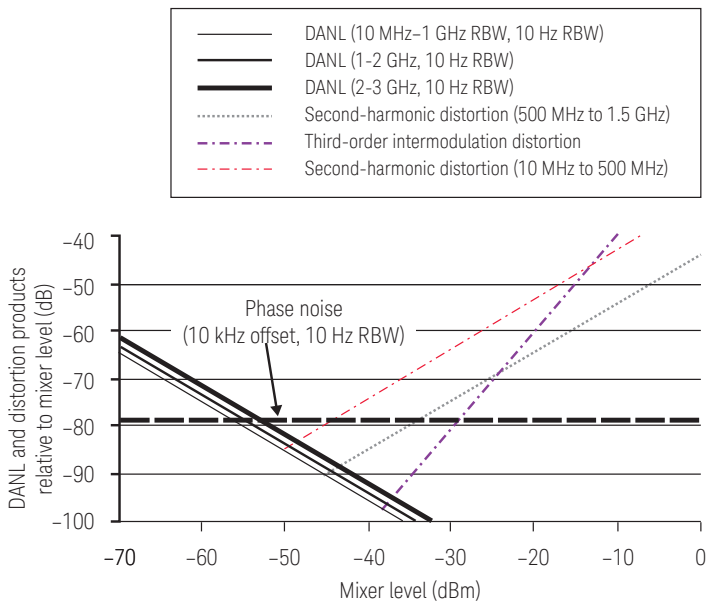
Figure 4. Sensitivity, phase noise, third-order intermodulation, and second-harmonic distortion versus mixer level for the Keysight E4402B
