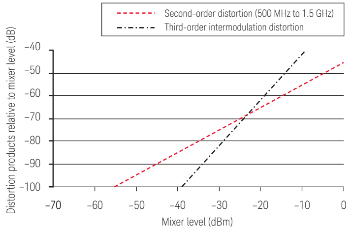
Figure 3. Internally generated second-harmonic and third-order intermodulation distortion levels as a function of mixer input level for the Keysight E4402B
