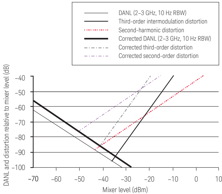
Figure 5. Dynamic range graph corrected for amplitude uncertainty
