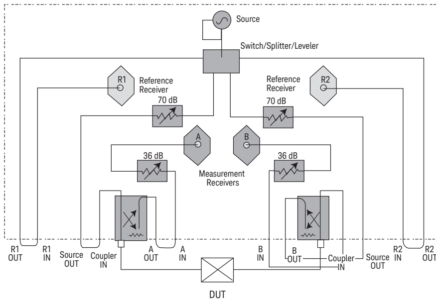
Figure 4. Re-configuration of the test set to further increase the dynamic range of the analyzer.
