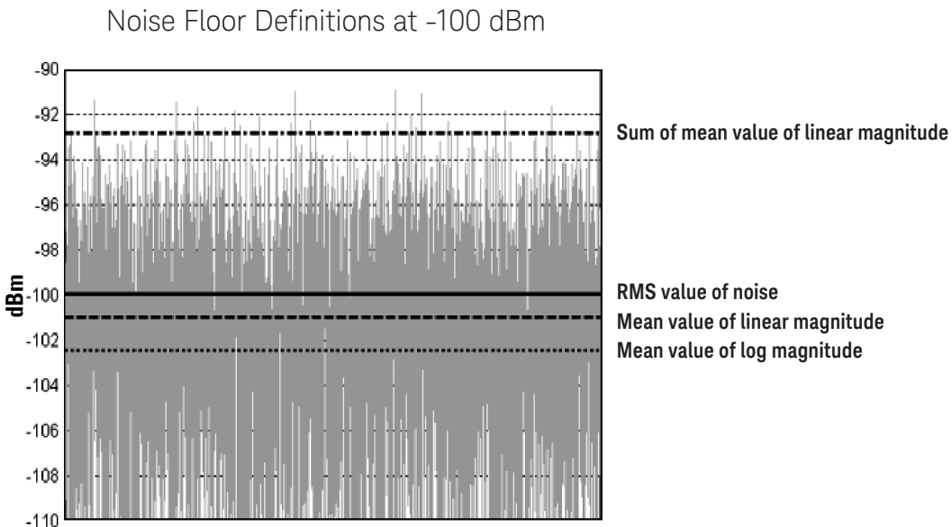
Figure 2. Various noise floor definitions
