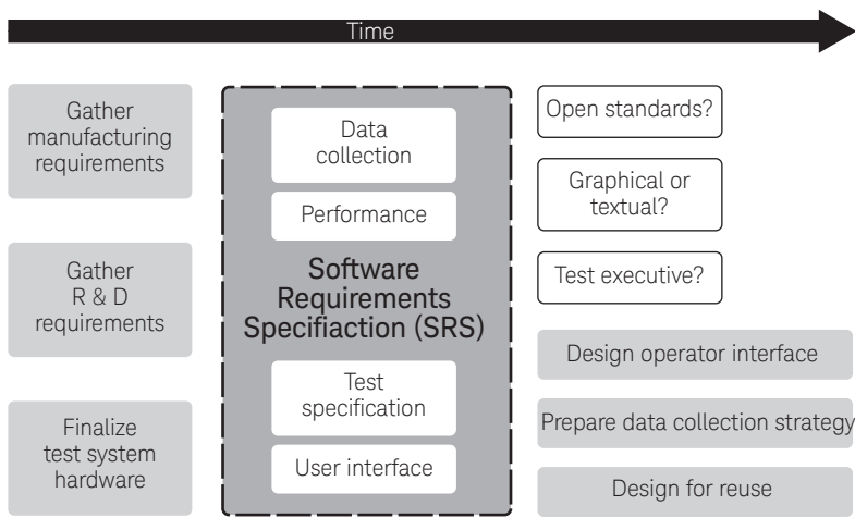
Figure 1. Test-system software development process overview
