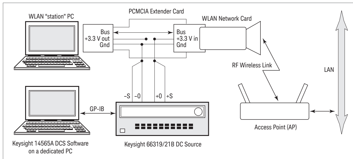
Figure 1. WLAN network card test set up configuration
