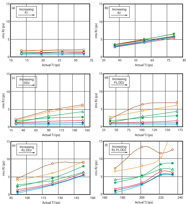
Figure 11: The RJ measurements as a function of TJ(10–12) for conditions dominated by (a) PJ, (b) RJ, (c) DDJ, (d) a mix of PJ*DDJ, (e) a mix of RJ*DDJ, and (f) a mix of PJ*RJ*DDJ.
