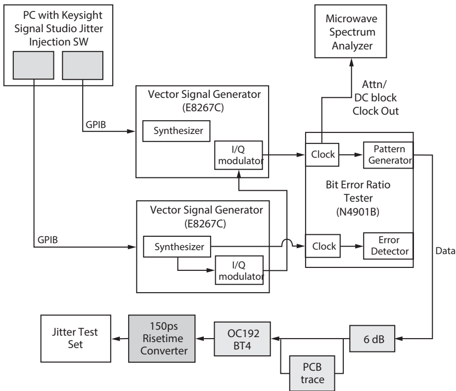
Figure 3: Block diagram of the precision jitter transmitter.
