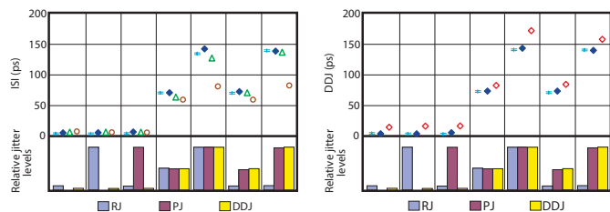
Figure 10: The (a) ISI and (b) DDJ measurements for an illustrative subset of conditions.
