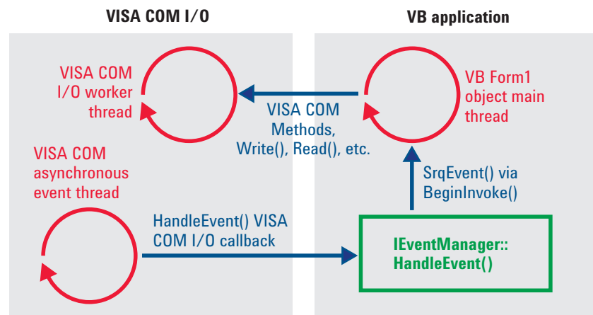
VISA COM I/O and VB threading
