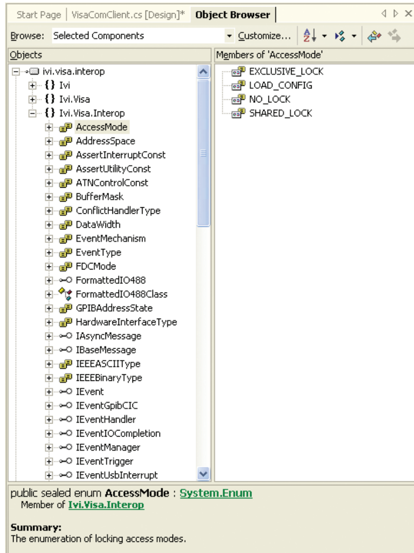
The Visual Studio Object Browser dialog
