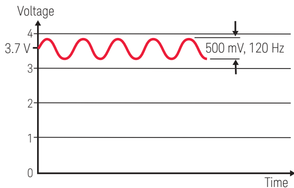
Figure 1. Example test waveform powering DC-to-DC converters
