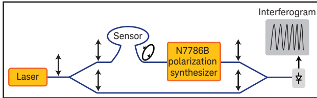
Figure 5. Interferometry/coherent detection
