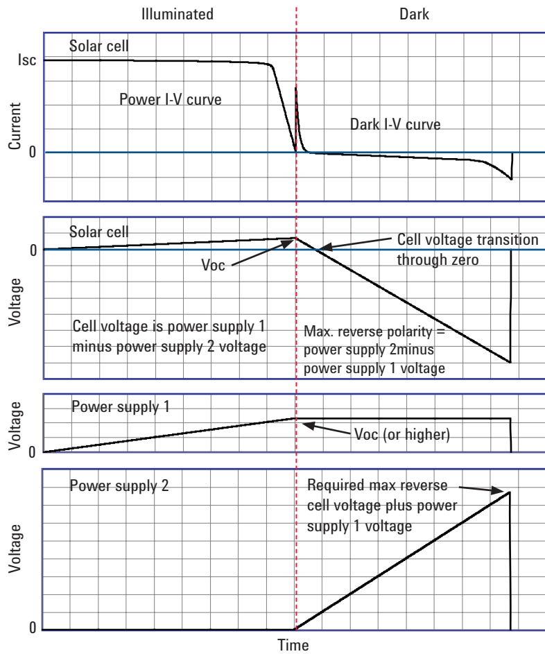
Figure 2. Solar cell voltage and current and the voltages of power supplies 1 and 2 plotted against time
