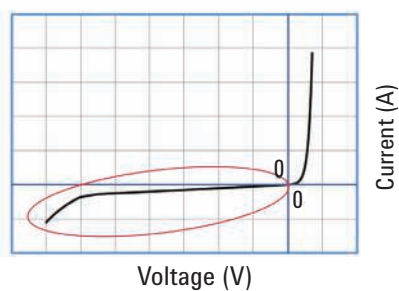
Figure 5: Dark I-V curve measurement (reverse bias region)
