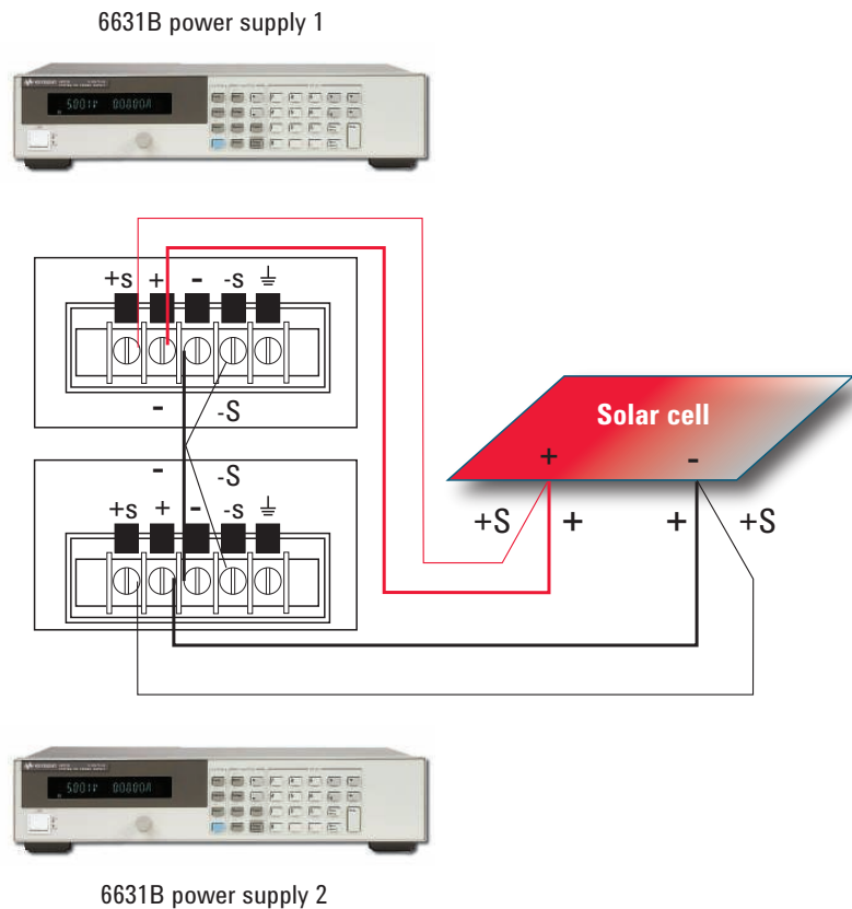
Figure 1: Two 6631B two-quadrant power supplies connected in anti-series
