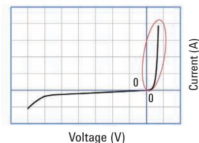
Figure 4: Dark I-V curve measurement (forward bias region)
