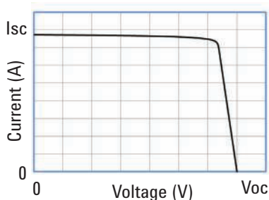
Figure 3: Illuminated cell I-V curve measurement (power quadrant)
