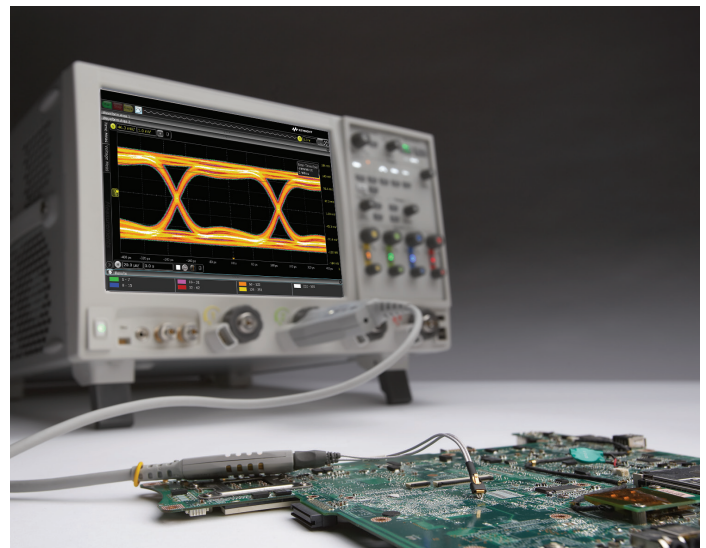
The InfiniiumMax III 30 GHz probing system includes accessories to enable probing with a ZIF tip, browsing, or connecting to 3.5 mm inputs.
