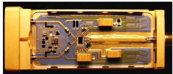
The InfiniiumMax III probing system uses the same InP technology that enables high bandwidth and low noise oscilloscope measurements.
