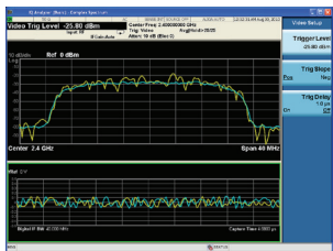
Figure 1. 40 MHz BW IQ waveform measurement
