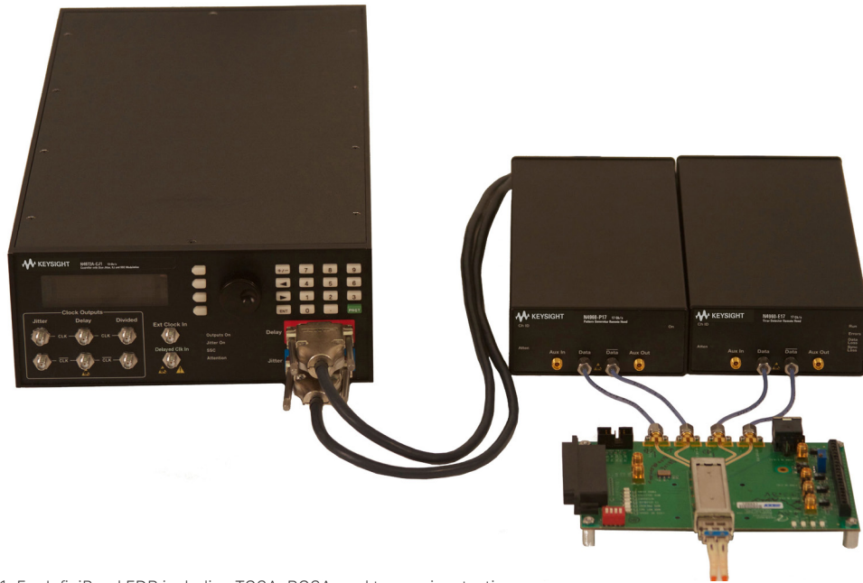
Figure 1. For InfiniBand EDR including TOSA, ROSA, and transceiver testing
