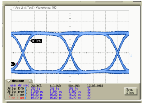
Figure 3. Typical eye at 14 Gb/s
