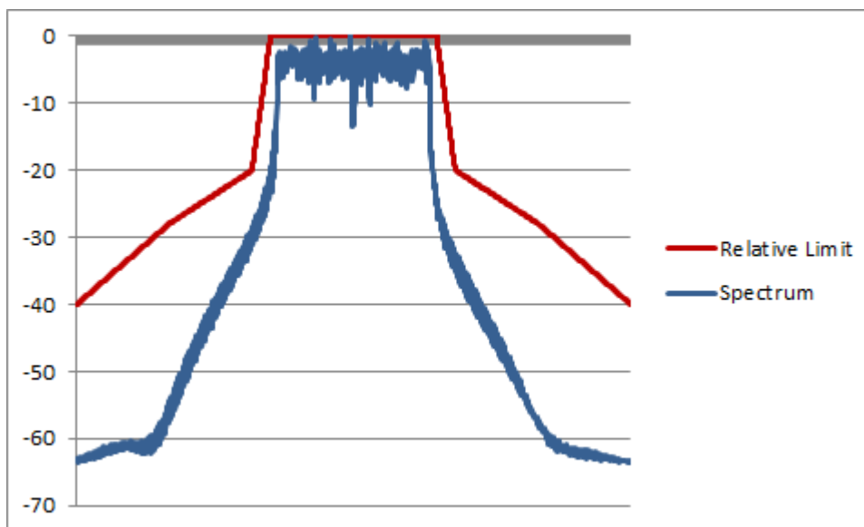
Figure 2. 802.11a/g SEM nominal performance at 5.8 GHz with 20 MHz bandwidth
