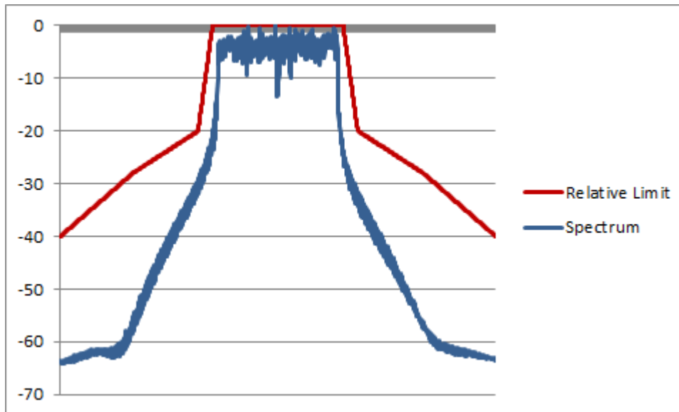
Figure 1. 802.11a/g SEM nominal performance at 2.4 GHz with 20 MHz bandwidth
