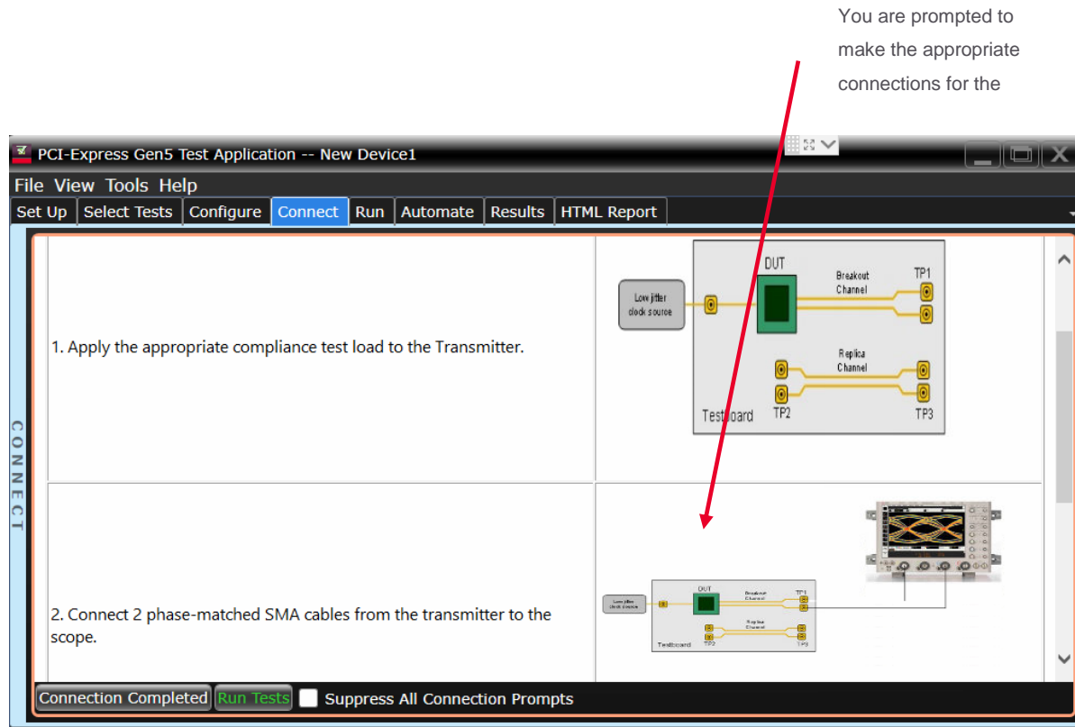
Figure 3. The D9050PCIC PCI Express 5.0 compliance application software includes connection diagrams to assist you with connecting your DUT to the oscilloscope.
