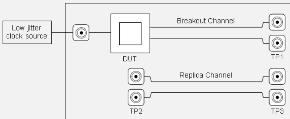
Figure 4. In order to test the transmitter of your PCIe 5.0 silicon, you will need to build or acquire a break-out board that allows you to connect high bandwidth test cables between your ASIC or DUT and your test instrumentation.
