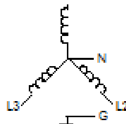
Three-Phase Wye with Neutral
