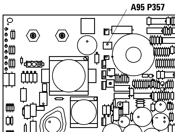
Figure 1. A95 Component Locator
