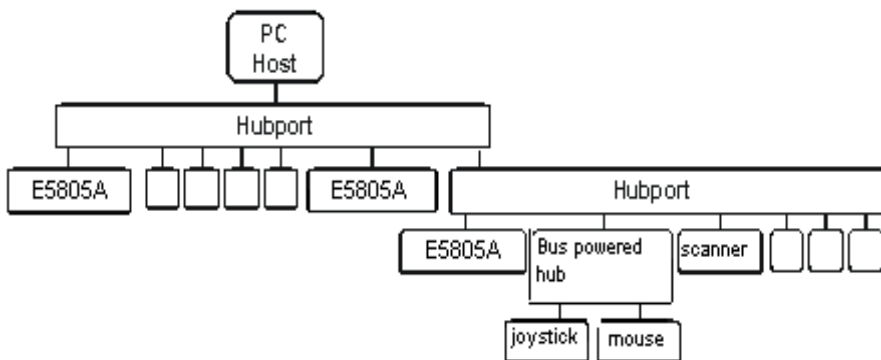
Figure 1 Hub Architecture
