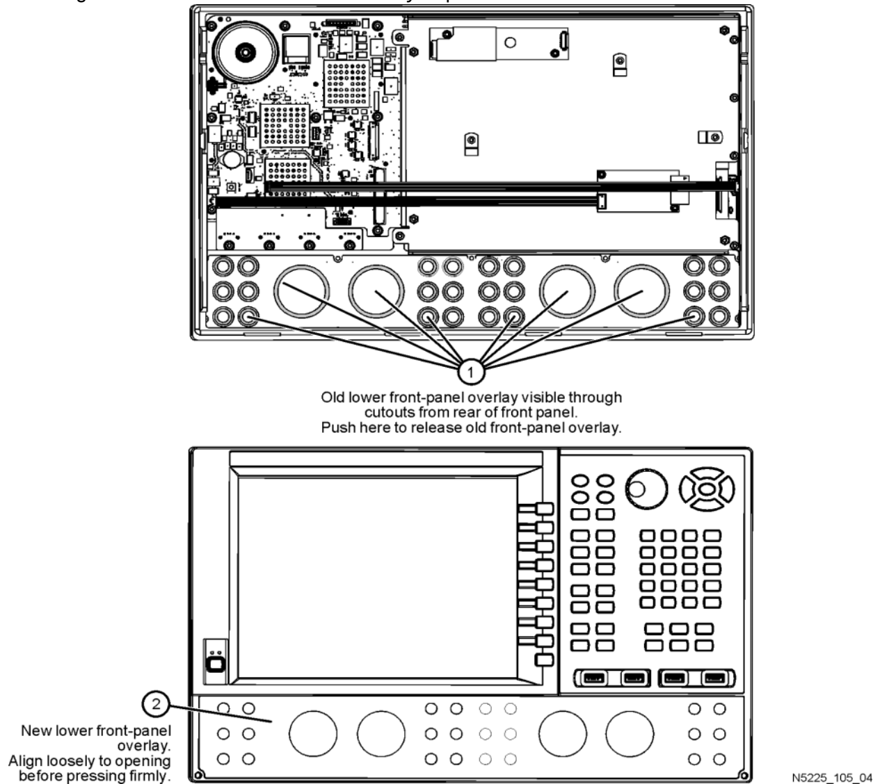
Figure 4 Lower Front Panel Overlay Replacement
