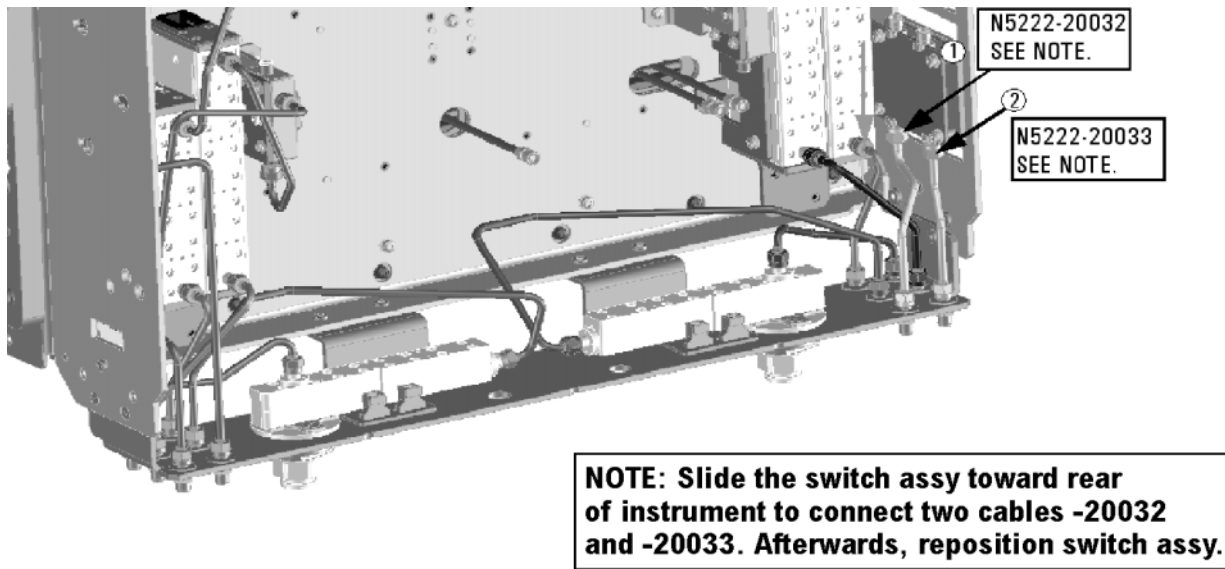
Figure 3 Instructions to Install W36
