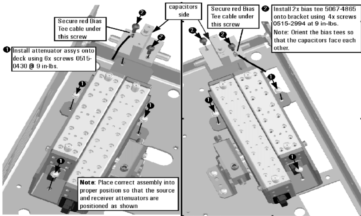
Figure 1 Bias Tees Installation
