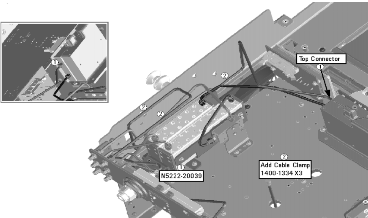
Figure 2 Location of Cable Clamps to Secure W40
