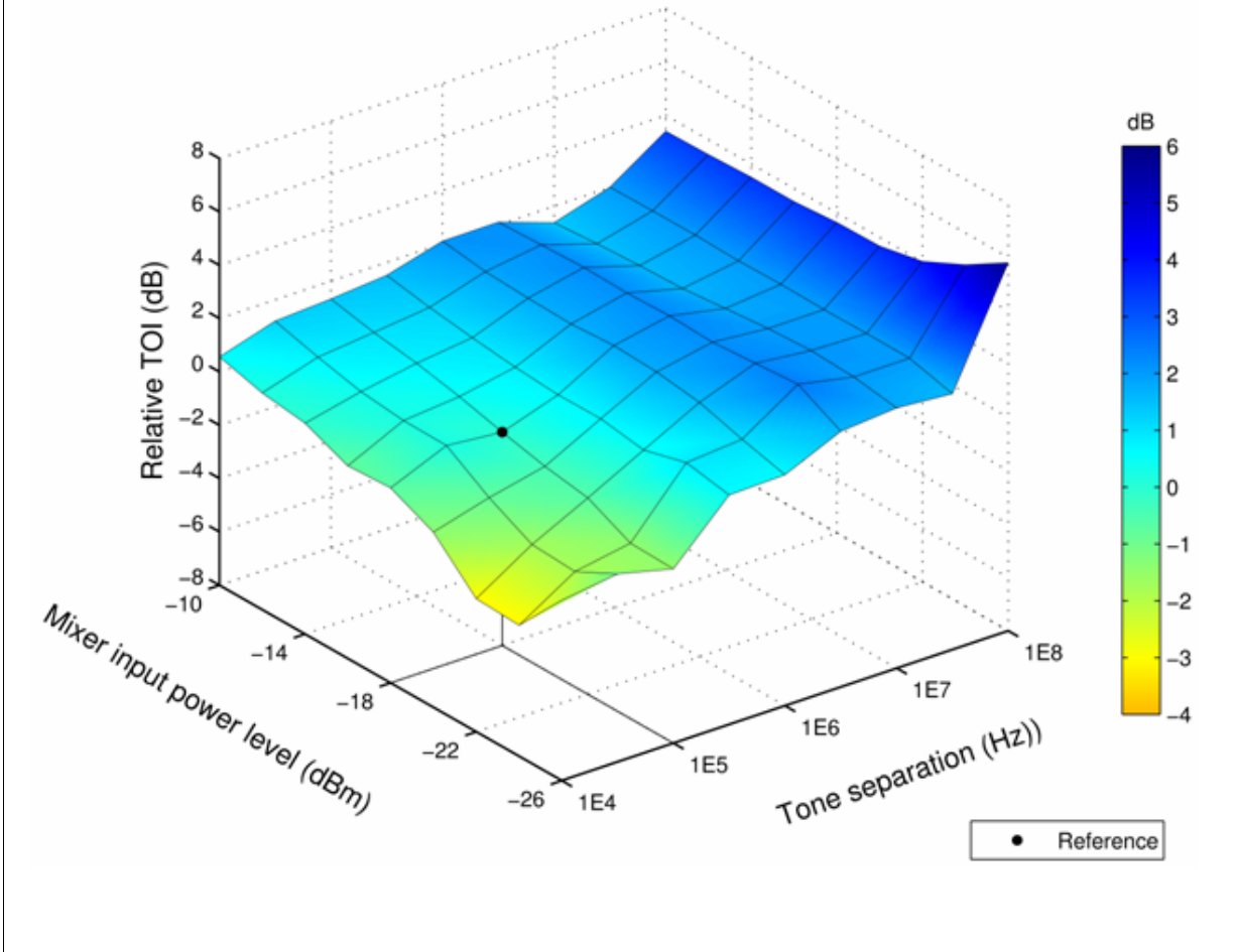
TOI vs. Mixer Level and Tone Separation (Referenced to TOI verification conditions)
