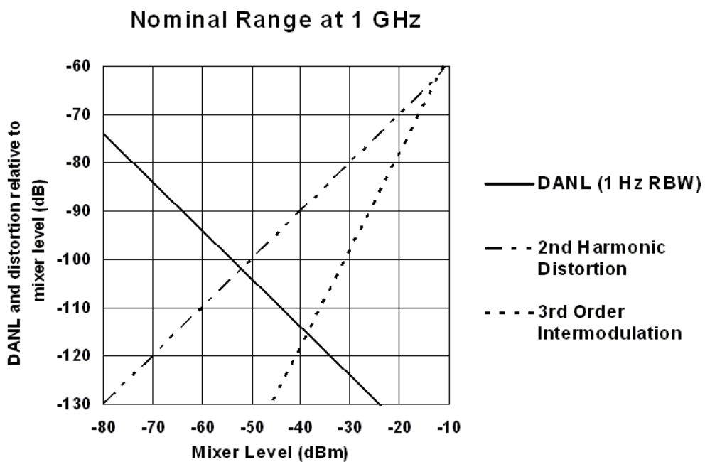
Nominal Dynamic Range at 1 GHz (Option 503, 508, 513, or 526) [Plot]
