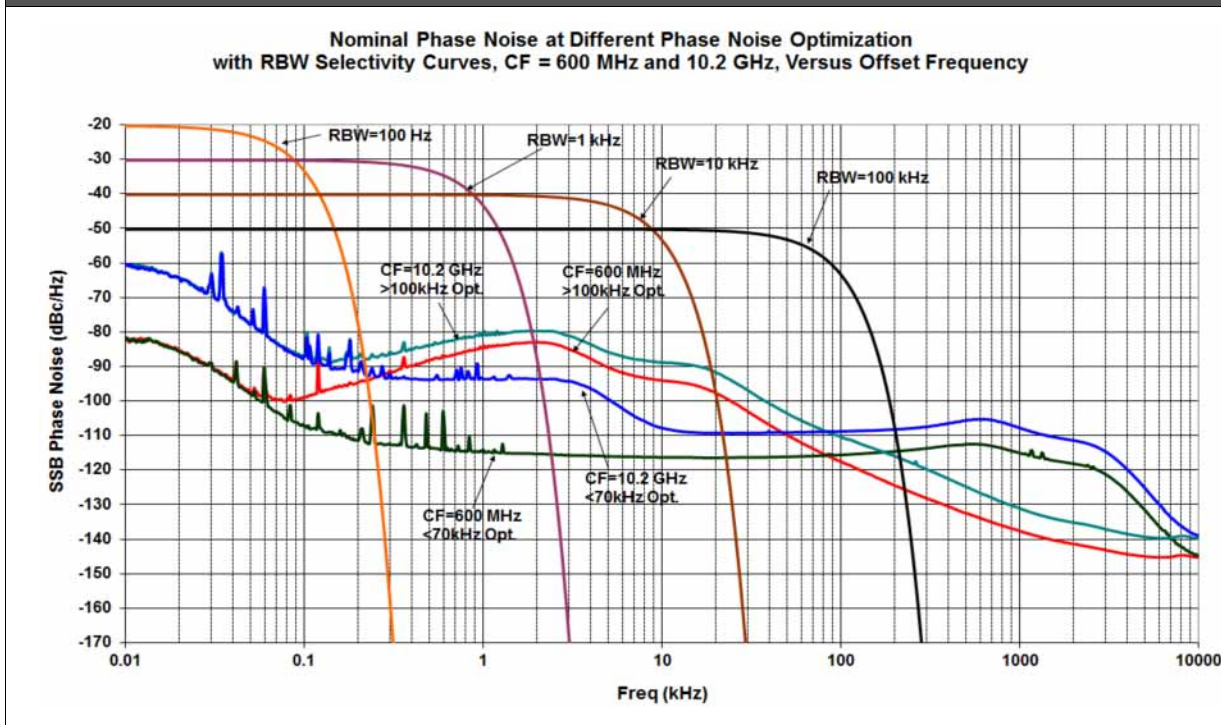
Nominal Phase Noise of Different LO Optimizations (Option 503, 508, 513, or 526) [Plot]
