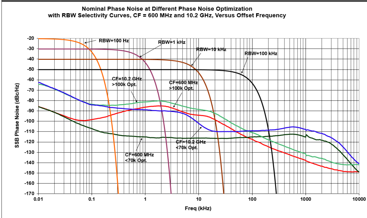
Nominal Phase Noise of Different LO Optimizations (Option 532, 544, or 550) [Plot]
