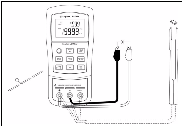
Figure 1-1 Capacitance measurement
