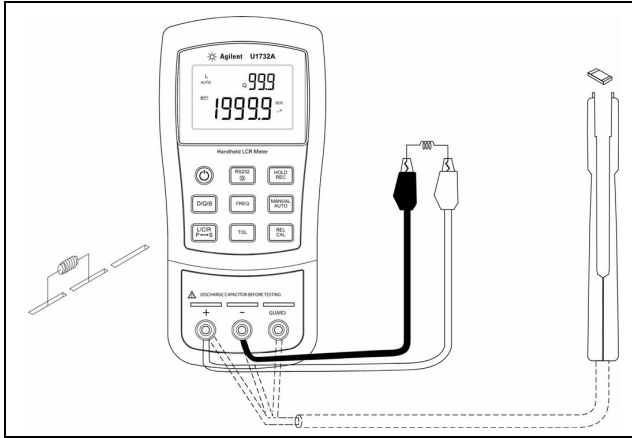
Figure 1-1 Inductance measurement
