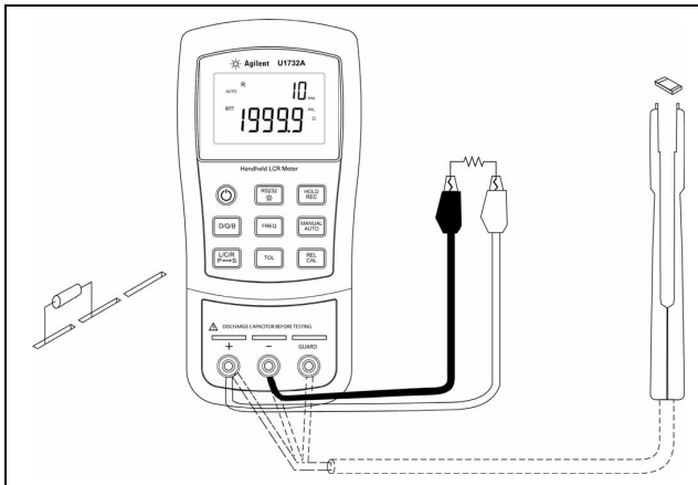
Figure 1-1 Resistance measurement
